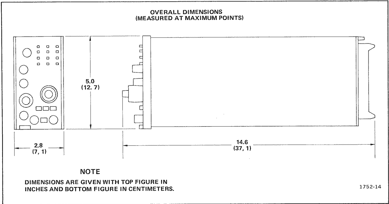
Fig. 1-2. Dimensional drawing.
