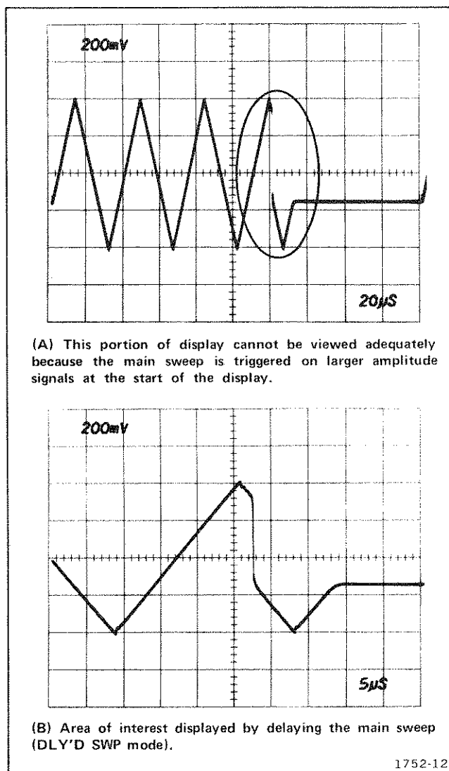
Fig. 2-11. Displaying a complex signal using delayed sweep.
