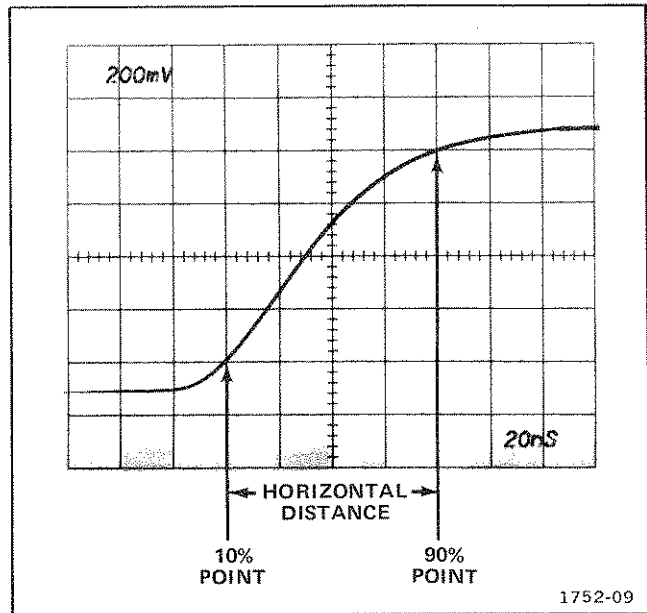
Fig. 2-8. Measuring risetime.
